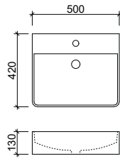
Iconic 500 With Overflow and Tap Landing
