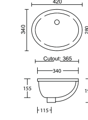
Oval Undermount Overflow to Front
