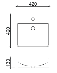
Iconic 420 With Overflow and Tap Landing
