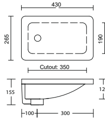
Mini Rectangle Undermount Overflow to Side
