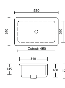
Rectangle Undermount Overflow to Back
